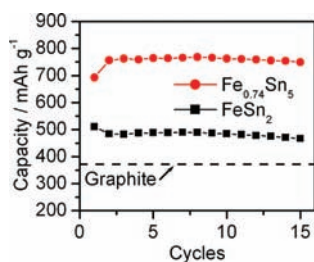
Figure 5. Reversible capacities of Fe 0.74 Sn 5 and FeSn 2 nanospheres as anodes in Li ion batteries.
