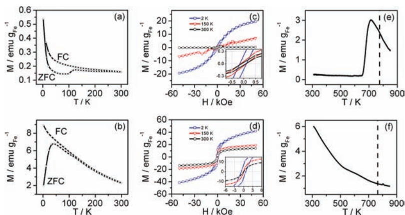
Figure 3. The temperature dependencies of the zero field cooled (ZFC) and field cooled (FC) magnetizations in applied fields of 0.05 kOe for (a) \text{Fe}_{0.74}\text{Sn}_5 and (b) \text{FeSn}_2 nanoparticles. The magnetic field dependencies of the magnetizations for (c) \text{Fe}_{0.74}\text{Sn}_5 and (d) \text{FeSn}_2 nanoparticles, where the insets are expanded views of the same magnetizations but at lower fields. The high-temperature part of the ZFC magnetizations in an applied field of 1 kOe for (e) \text{Fe}_{0.74}\text{Sn}_5 and (f) \text{FeSn}_2 nanoparticles, where the dashed lines indicate the melting points determined from DTA measurements.
